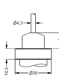
cable outlet with PVC cable (IP 67) 6
