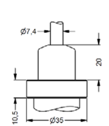
cable outlet, cable with ventilation tube (IP 68) 7
