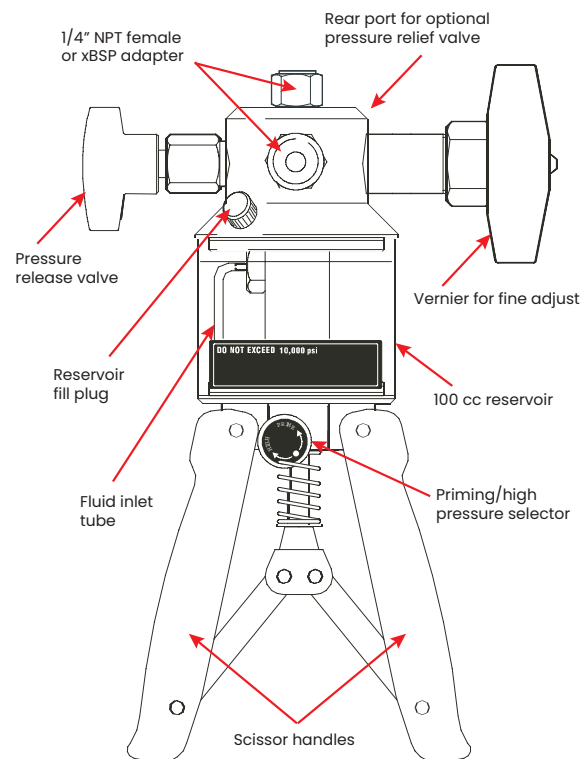
PV212-X components
