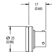
MIL-C-26482 (6 PIN SHELL SIZE 10)
