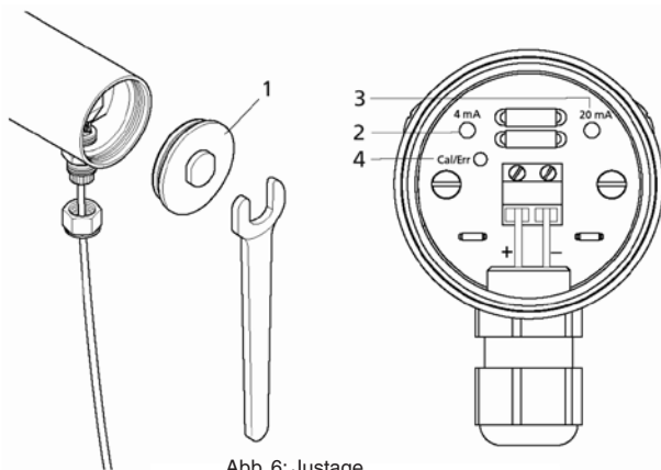
Abb. 6: Justage
