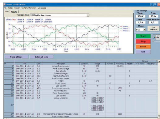
PQ Meter Test Program control panel
