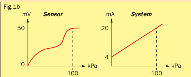
Exemple of a system (sensor + transmitter) with an output linear to the process value, in spite of a non-linear sensor.
