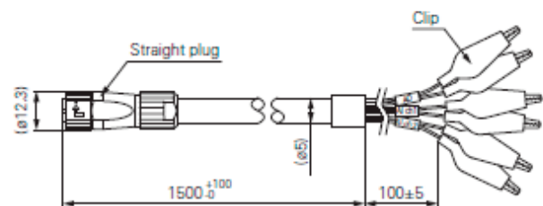
Detector FSDP (Detector for flow velocity profile measurement)
