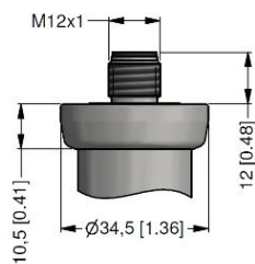
M12x1 (5-polig)
