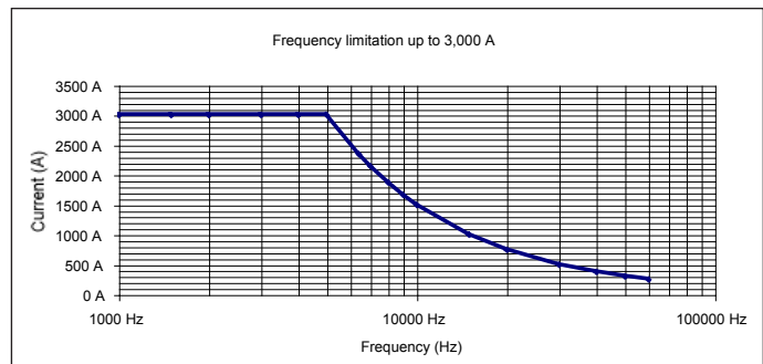
(6) Frequency limitation according to amplitude
