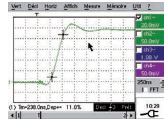
Pulse response
