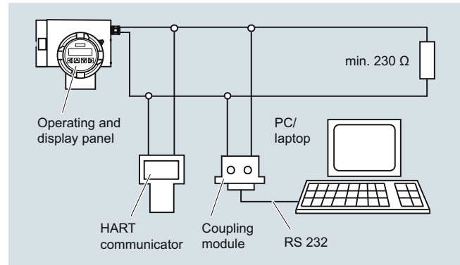
HART communication
