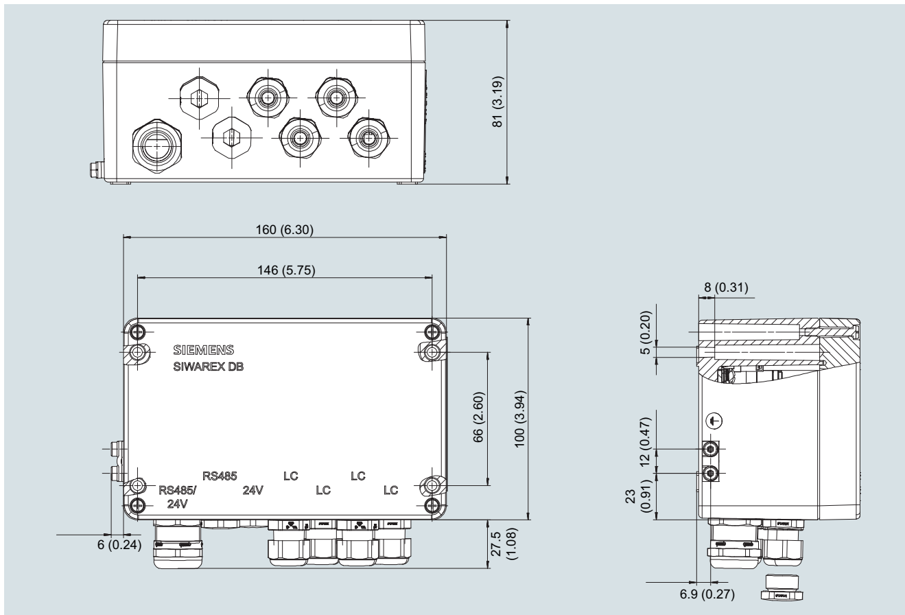
SIWAREX DB digital junction box (7MH5001-0AD20), dimensions in mm (inch)
