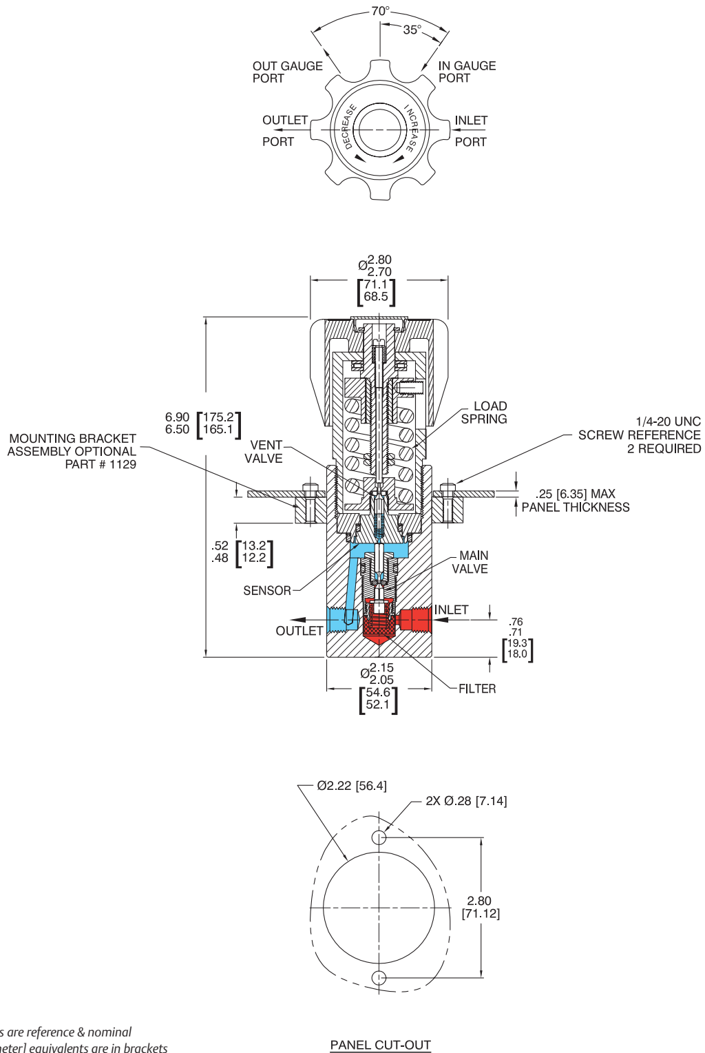
PANEL CUT-OUT
