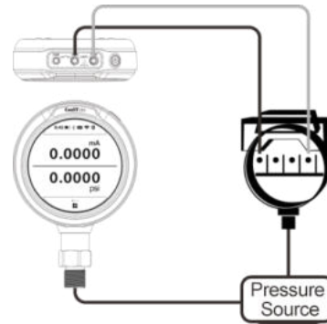
Figure 13 Calibrate pressure transmitter
