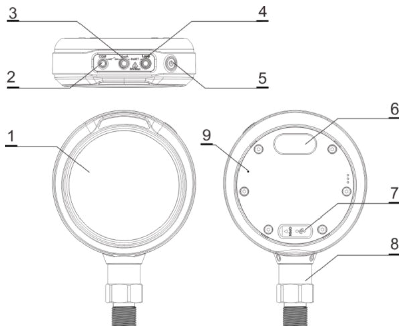
Figure 1 Basic Structure
