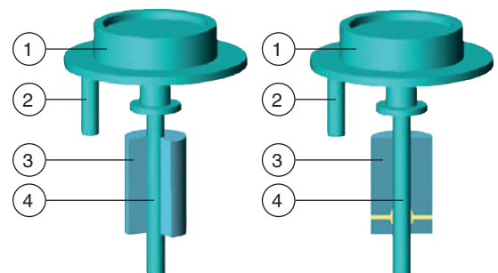
Fig. left: Oil-operated piston-cylinder system
