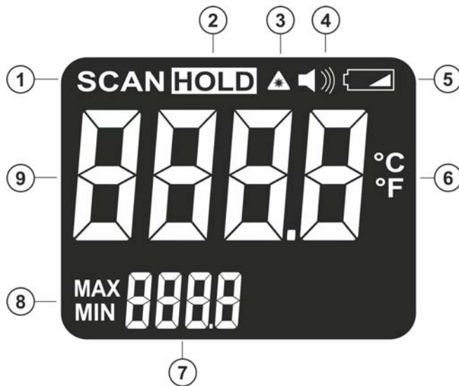
Fig. 3: LCD display description
