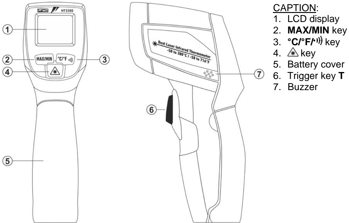
Fig. 1: Description of the instrument's front and lateral sides
