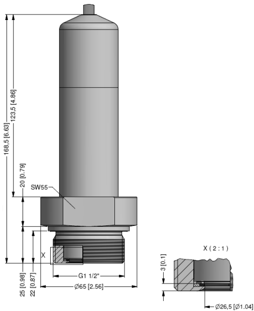
screw-in version
