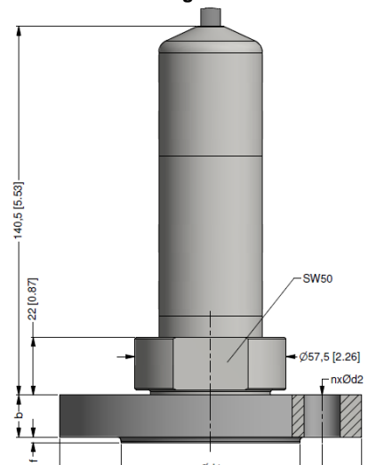
flange version
