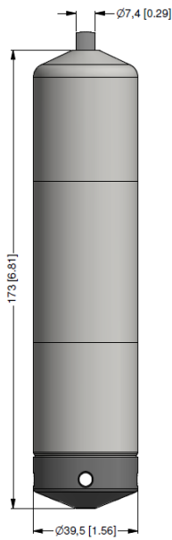
screw-in version
