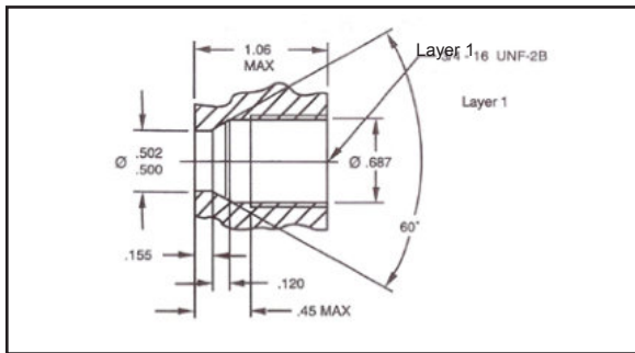
Figure 1: PT375 Mounting Hole Diagram
