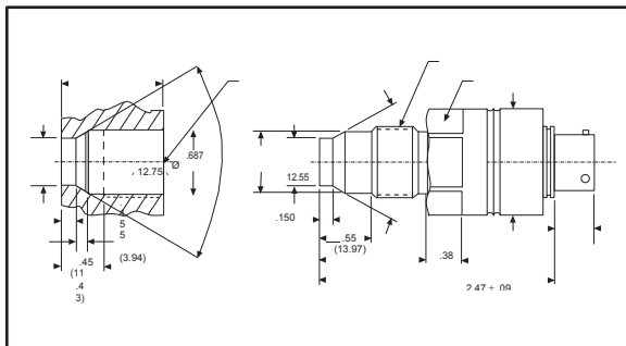
Figure 2: PT375 Schematic
