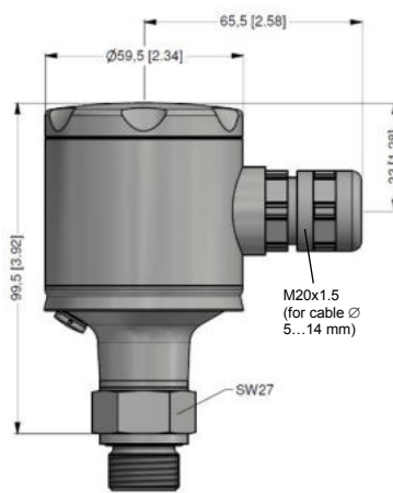
universal field housing (IP 67)
