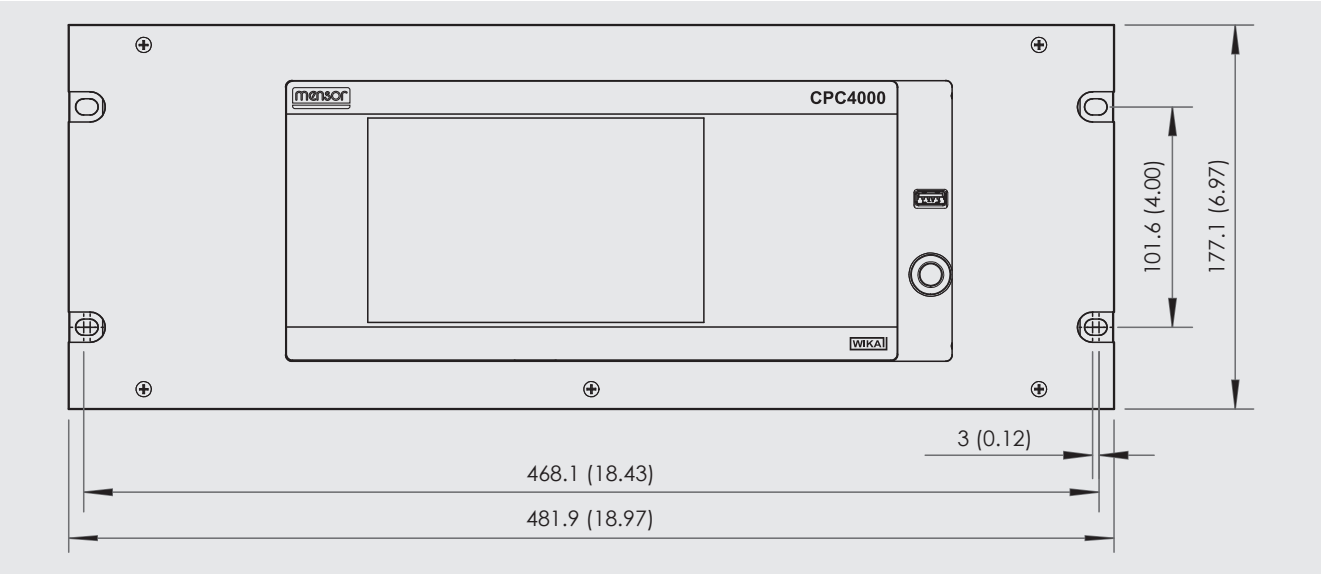
19" rack-mounting kit, front view
