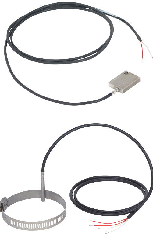
Fig. top: Model TR50 with metal contact block Fig. bottom: Model TR50 with tightening strap
