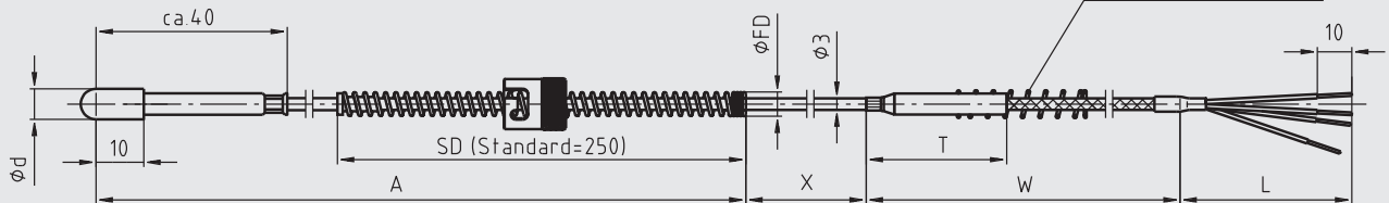
Probe tip, round
