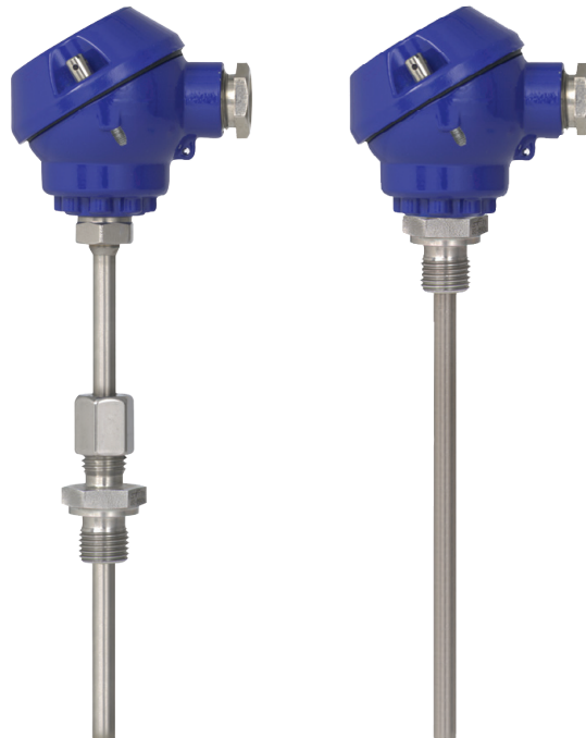
Fig. left: Model TC10-D with process connection compression fitting
