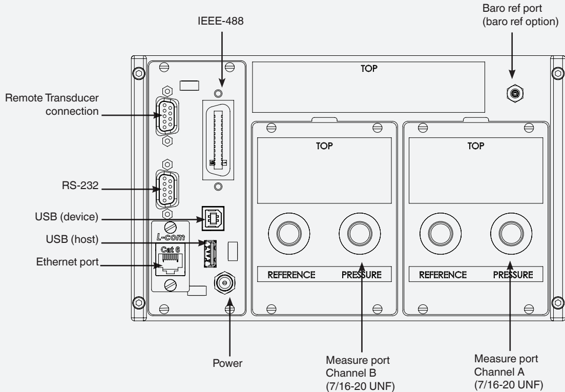
Rear Panel
