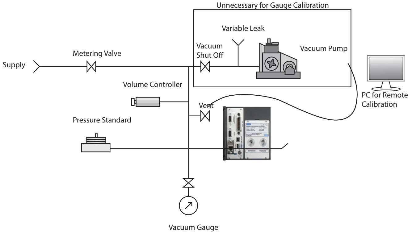
Figure 10.4 - Calibration Setup
