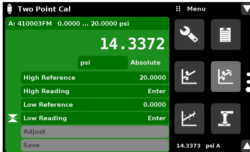
Figure 10.8-B “High Reading” and “Low Reading”
