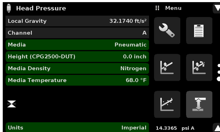
Figure 10.10-C Pressure values (Channel A)
