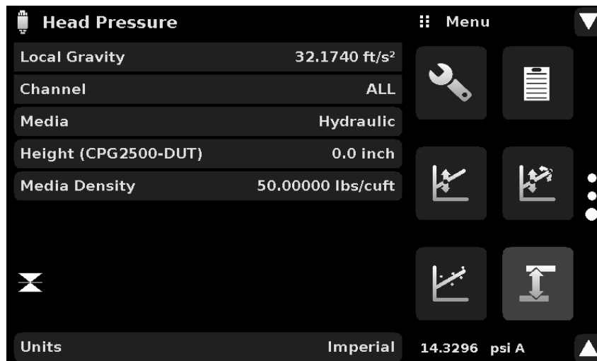
Figure 10.10-D - Head Pressure, Hydraulic
