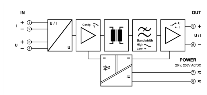
Block diagram
