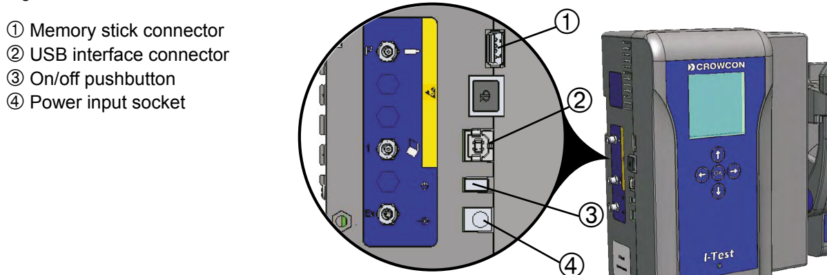
Figure 3: Electrical connections & controls
