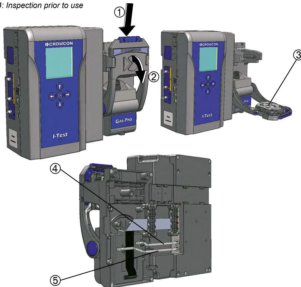
Figure 4: Inspection prior to use
