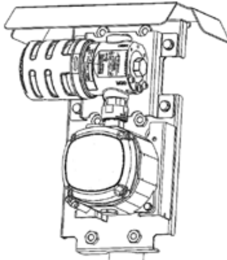
Figure 19: IR Plus Junction Box Mounting
