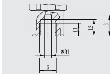
EN 837, female thread
