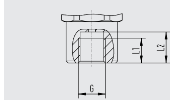
Female thread, compatible with bite-type fitting
