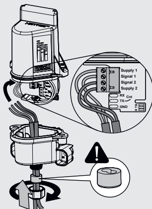
Connecting a dual analogue connection
