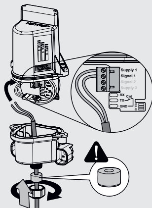
Connecting a single analogue connection
