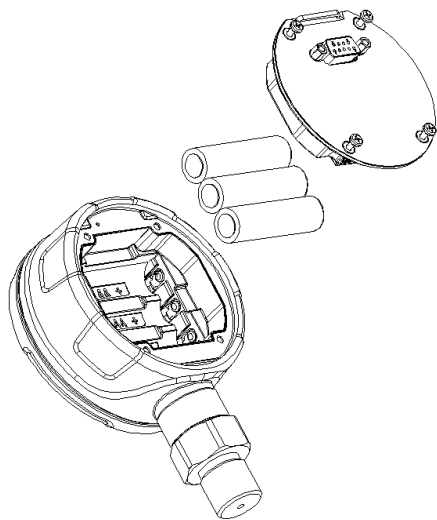
Figure 3 Install batteries
