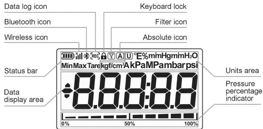
Figure 5 Main Display
