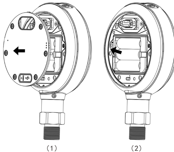
Figure 3 Battery installation
