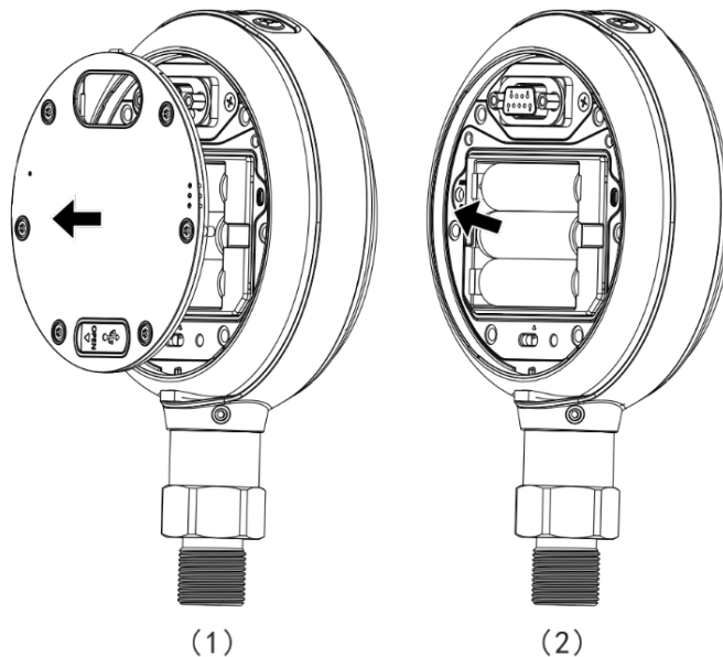
Figure 2-2 Power supply by battery
