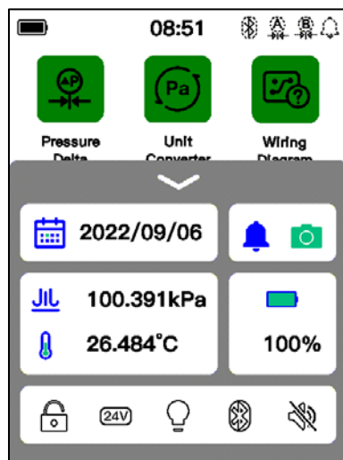
Figure 4 Control center
