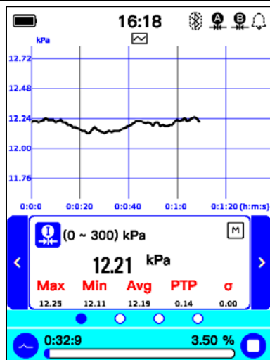
Figure 11 Single-channel mode
