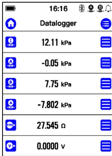
Figure 5 Calibrator main screen
