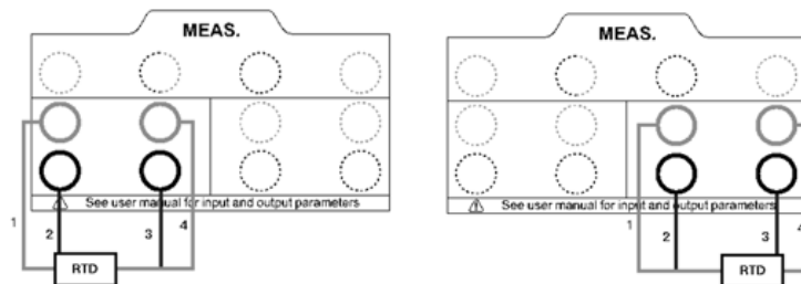
Figure 6 RTD measurement
