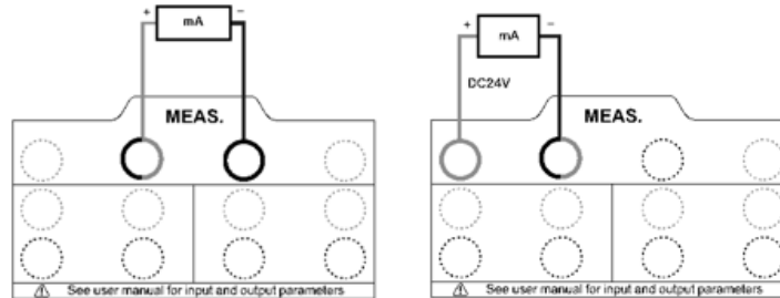
Figure 8 Current measurement
