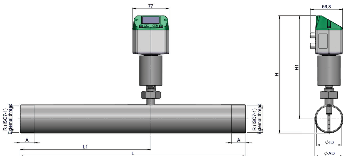
IVD 520- with thread
