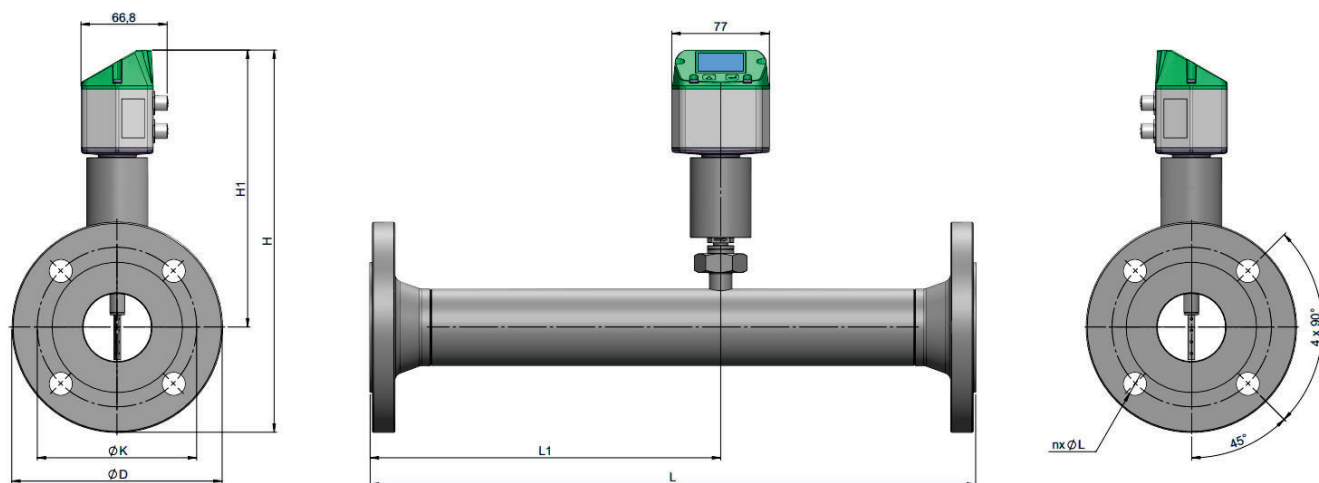
IVD 520 - with flange (Material stainless steel: 1.4404)
