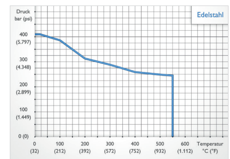
Manometer-Siphon
