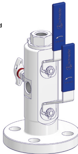
Double Isolate Ball Valve and Single Vent Needle Valve
