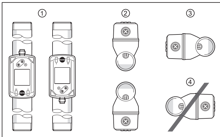
Fig. 1: Orientation of the pipe length and the unit
